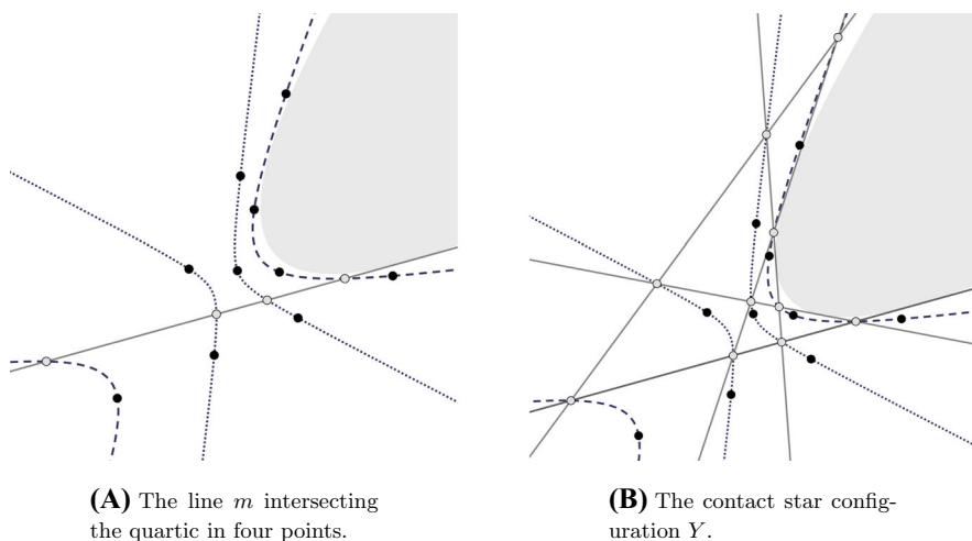
Figure 4. Construction of the set of points X \cup Y on a reduced quartic
