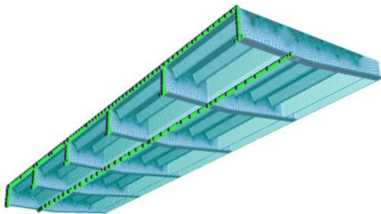
Figure 14. Representation of the shell structural model for nominal stress assessment in the connection details carried out with the MIDAS GEN ® software (version GEN2021 v3.2, MIDAS Information Technology Co.Ltd., Milan, Italy).
