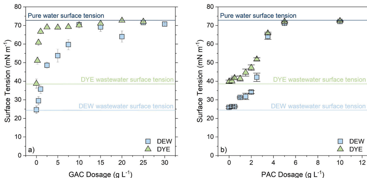
Fig. 2. Effect of activated carbon adsorption on the surface tension of textile industry wastewaters. Batch adsorption tests were performed using (a) granular activated carbon (GAC) and (b) powdered activated carbon (PAC) at increasing dosages. Surface tension was measured after 24 h of contact. The surface tension of pure water ( 72.7 \text{ mN m}^{-1} at 20^\circ \text{C} ) is shown as a reference and represented by a horizontal blue line, while the surface tension of the untreated wastewaters is also reported for comparison. Error bars represent one standard deviation based on two independent, replicate tests. (For interpretation of the references to color in this figure legend, the reader is referred to the web version of this article.)
