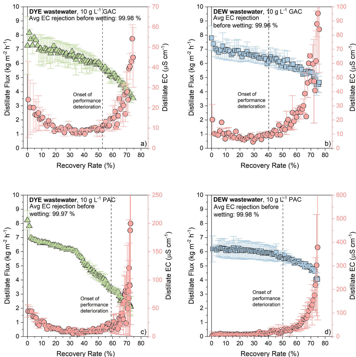
Fig. 4. Performance of direct contact membrane distillation (DCMD) treating textile wastewaters pre-treated by adsorption with activated carbon at a dosage of 10 g L -1 . Panels (a) and (b) report results for dyeing (DYE) and dewatering (DEW) wastewaters, respectively, pre-treated with granular activated carbon (GAC), while panels (c) and (d) show the corresponding results for wastewaters pre-treated with powdered activated carbon (PAC). Distillate flux (left y-axis) and distillate electrical conductivity (EC, right y-axis) are presented as a function of recovery rate. The vertical dashed line indicates the onset of membrane wetting, defined as the first recovery at which distillate EC showed a sustained increase above the stable baseline (Section 2.4). Error bars represent one standard deviation based on two independent, replicate tests.
