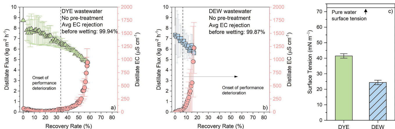
Fig. 1. Results of direct contact membrane distillation tests performed on raw textile industry wastewaters. The evolution of distillate flux (left y-axis) and distillate electrical conductivity (EC, right y-axis) as a function of recovery rate is shown for wastewaters from (a) the dyeing process (DYE) and (b) the synthetic fiber dewatering (DEW) process. Experiments were carried out without pre-treatment. The vertical dashed line indicates the onset of membrane wetting, defined as the first recovery at which distillate EC showed a sustained increase above the stable baseline (Section 2.4). Error bars represent one standard deviation based on two independent, replicate tests. Panel (c) reports the initial surface tension of the two wastewaters.
