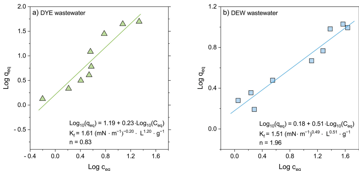
Fig. 3. Granular activated carbon adsorption isotherms obtained for (a) dyeing (DYE) wastewater and (b) dewatering (DEW) wastewater. Symbols denote experimental equilibrium data, reported as adsorbed amount at equilibrium ( q_{eq} ) versus equilibrium concentration in solution ( C_{eq} ). Solid lines represent the Freundlich model fitted to the data, expressed in its nonlinear form as q_{eq} = K_F C_{eq}^{\frac{1}{n}} , and in the linearized logarithmic form as \text{Log}_{10} q_{eq} = \text{Log}_{10} K_F + \frac{1}{n} \text{Log}_{10} C_{eq} . The corresponding linear regressions, along with the estimated Freundlich parameters K_F and n , are reported within each panel. Both isotherms are presented on logarithmic coordinates.
