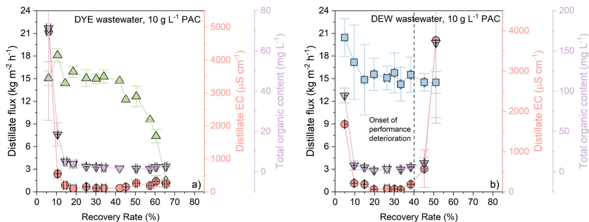
Fig. 5. Performance of vacuum membrane distillation (VMD) treating textile wastewaters pre-treated by adsorption with powdered activated carbon (PAC, 10 g L -1 ). Panels (a) and (b) report results for dyeing and deweighting wastewaters, respectively, showing distillate flux (left y-axis), and distillate electrical conductivity and total organic content (EC, red right y-axis and TOC, purple right y-axis respectively) as a function of recovery rate. Lines connecting data points are solely meant as a guide for the eye. The vertical dashed line indicates the onset of membrane wetting, defined as the first recovery at which distillate EC showed a sustained increase above the stable baseline (Section 2.4). Error bars represent one standard deviation based on two independent, replicate tests. (For interpretation of the references to color in this figure legend, the reader is referred to the web version of this article.)
