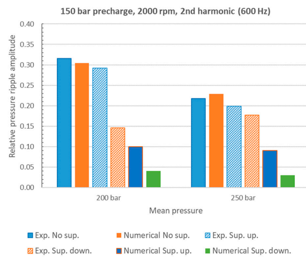
Figure 12. FFT of the pressure ripple, 2nd harmonic, pump speed = 2000 rpm.
