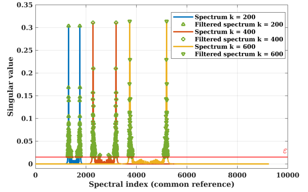
Fig. 4: Spectrum of the \mathbf{C} - \mathbf{C}_c for increasing frequencies.
