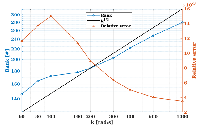
Fig. 5: Accuracy of the solution and rank of the compressed matrix as a function of k , with a compression parameter \varepsilon = 0.015 .
