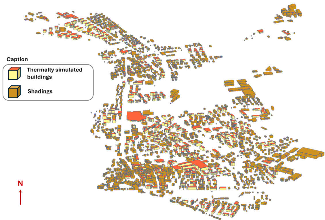
Fig. 3. Whole UBEM for the city of Monthey.
