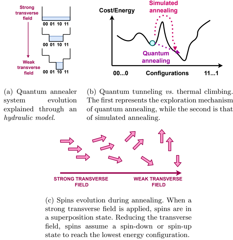
Fig. 4: Overview of quantum annealing.
