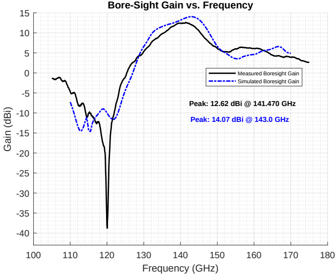
Fig. 5. FP antenna boresight gain.
