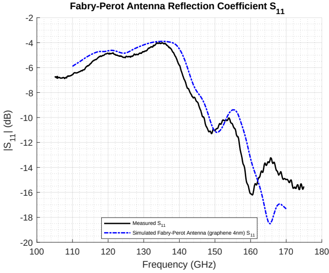
Fig. 6. FP antenna reflection coefficient.
