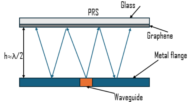
Fig. 4. Conceptual model of FP antenna.
