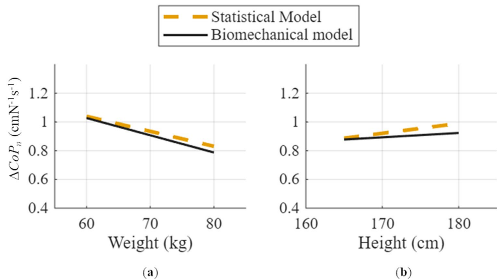
Fig. 8 Comparison between the statistical and biomechanical models. a CoP trend as the subject weight changes (height = 172 cm); b CoP trend as the subject height changes (weight = 70 kg)
