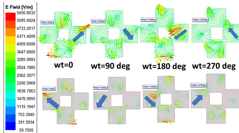
Figure 5. Simulated field snapshots at different time phases (at \omega t = 0^\circ, 90^\circ, 180^\circ, 270^\circ ) showing LHCP (top row) and RHCP (bottom row) for the two feed configurations of Figure 6 at 28.2 GHz.
