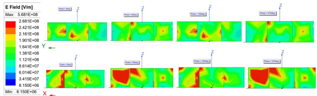
Figure 4. Eigenmode Mag- E of the cross-shaped dielectric resonator at \omega t = 0^\circ, 90^\circ, 180^\circ, 270^\circ on the YZ (top) and XZ (bottom) planes, indicating a perturbed/hybrid TE-like mode derived from the quasi- TE_{311} family.
