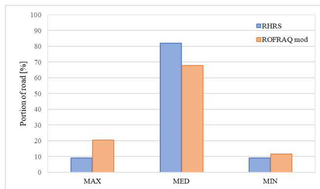
Figure 4. Percentage distribution of road sections falling into the three different risk levels.
