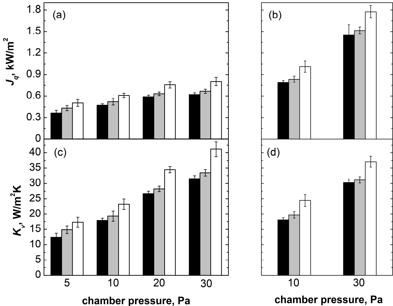
Figure 2. J_q and K_v as a function of P_C and T_S for (■) central, (▒) semi-border, and (□) border vials in direct contact with the shelf. Data reported in (a) and (c) refer to T_S = -10\text{ }^\circ\text{C} for various chamber pressures; data reported in (b) and (d) refer to T_S = +10\text{ }^\circ\text{C} for P_C = 10\text{ Pa} and T_S = +30\text{ }^\circ\text{C} for P_C = 30\text{ Pa} .
