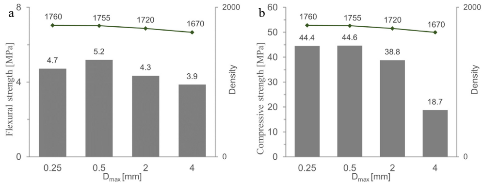
Fig. 2. (a) influence of the maximum aggregate diameter on the flexural strength of foamed concrete with a target dry density equal to 1750 \pm 50 kg/m³; (b) influence of the maximum aggregate diameter on the compressive strength.
