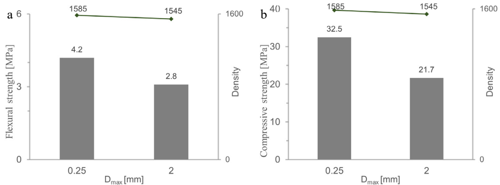
Fig. 3. (a) influence of the maximum aggregate diameter on the flexural strength of foamed concrete with a target dry density equal to 1550 \pm 50 kg/m³; (b) influence of the maximum aggregate diameter on the compressive strength.
