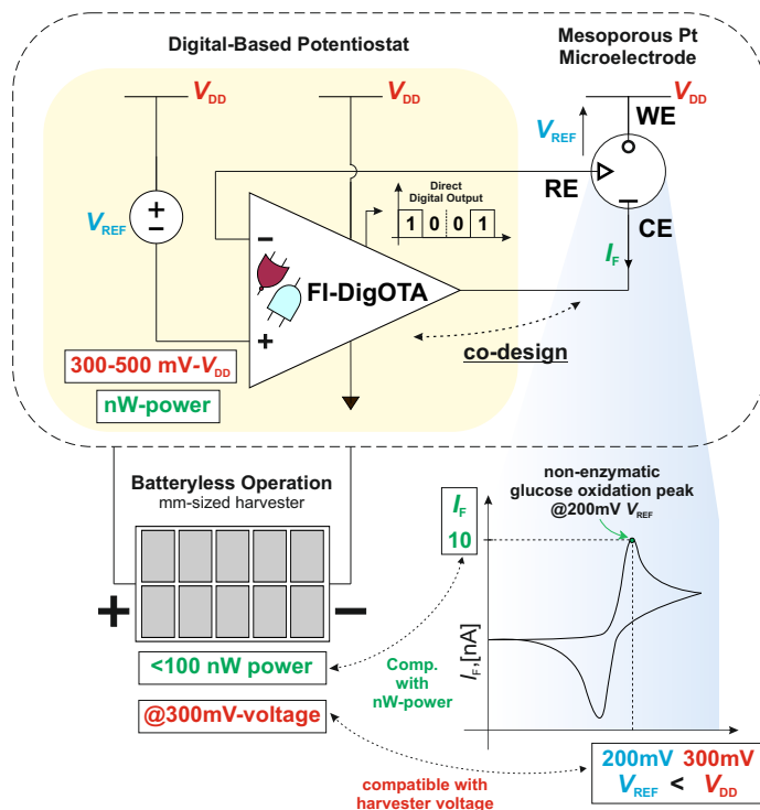
Fig. 1: Electrochemical-biosensor constraints for non-enzymatic glucose detection addressed by the proposed DB potentiostat and mesoporous platinum (Pt) microelectrode co-design.
