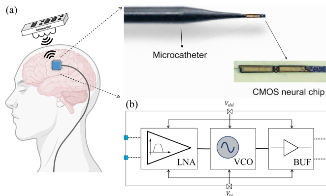
Fig. 1: a) Conceptual illustration of the intravascular probe, where a CMOS neural chip is mounted at the tip of a microcatheter. The inset shows a zoomed view of the chip. b) System-level block diagram of the proposed neural recorder based on frequency-domain encoding and body-coupled communication.
