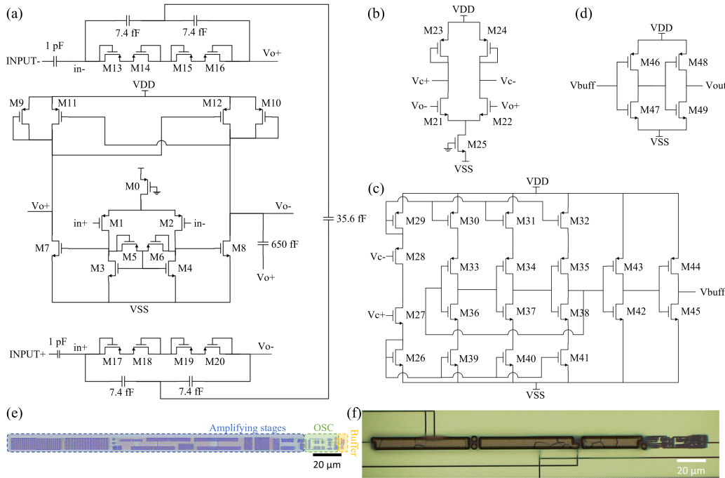
Fig. 2: Schematic of the a) LNA, b) diode-based amplifier for balancing the load of LNA, c) voltage-controlled oscillator and d) buffer to drive the system's load. e) System layout, and f) microphotograph of the fabricated circuit. Supply rails ( V_{DD} = +0.6 V, GND = 0 V, V_{SS} = -0.6 V) are externally supplied DC biases, intended to be delivered through the catheter in the target application.
