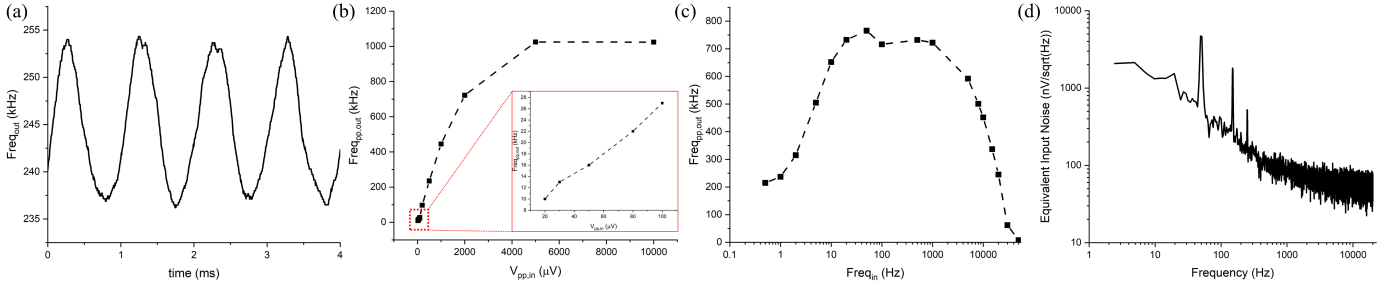
Fig. 3: Measured system performance: (a) instantaneous output frequency for a 50 \mu V pp , 1 kHz sinusoidal input; peak-to-peak frequency deviation versus (b) input amplitude and (c) input frequency; and (d) equivalent input-referred noise spectral density of the complete frequency-encoding front end.
