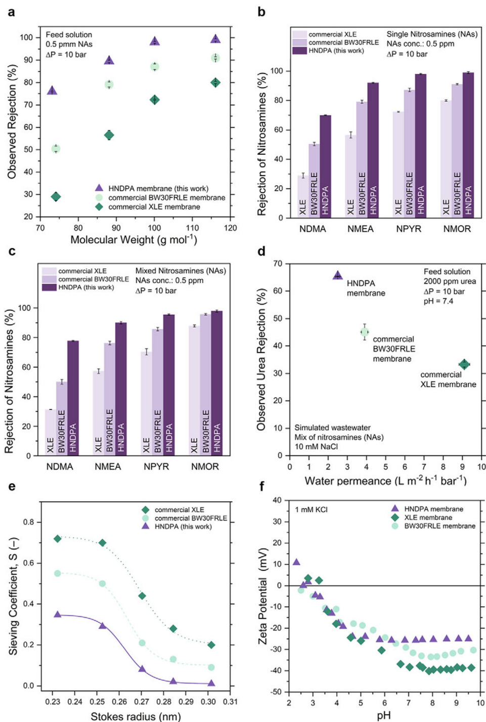
Figure 2. Molecular selectivity of the HNDPA membrane. (a) Rejection of individual nitrosamines as a function of molecular weight for the HNDPA membrane and for two commercial reverse osmosis membranes (XLE, BW30FRLE). Nitrosamine rejection for single-solute (b) and mixed-solute (c) feeds. All filtration experiments were conducted at a total nitrosamine concentration of 500 \mu\text{g L}^{-1} , an applied pressure of 10 bar, and a feed temperature of 25 \pm 2^\circ\text{C} . (d) Relationship between pure water permeance and urea rejection measured at a urea concentration of 2,000 \text{ mg L}^{-1} at 10 bar applied pressure. (e) Sieving coefficient ( S ) as a function of solute Stokes radius derived from neutral solute rejection experiments. (f) Zeta potential profiles of HNDPA, XLE, and BW30FRLE membranes plotted as a function of pH in 1 mM KCl.
