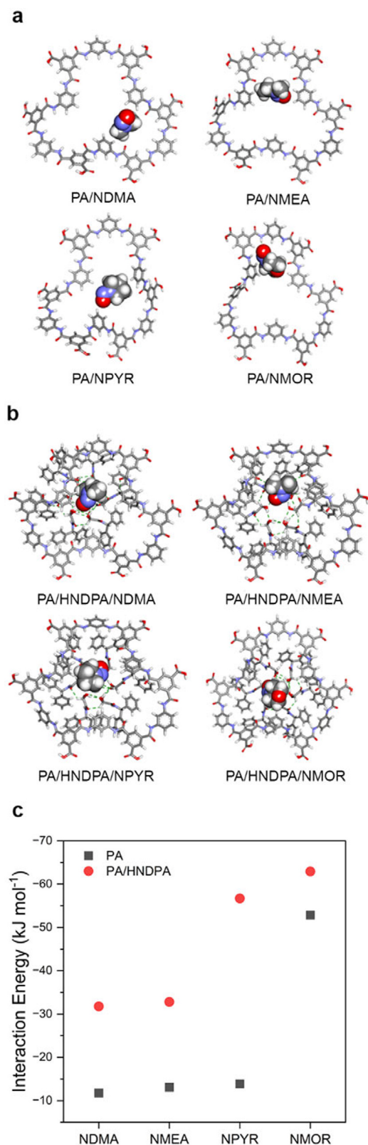
Figure 4. Molecular interactions between polyamide networks and nitrosamine contaminants. (a) Energy-minimized structures of polyamide (PA) interacting with representative nitrosamine molecules (NDMA, NMEA, NPYR and NMOR). (b) Corresponding equilibrated structures of polyamide/HNDPA system, highlighting the modified polymer network and the interaction with the pollutant molecules. (c) DFT-calculated interaction energies for pristine polyamide and polyamide/HNDPA with each nitrosamine.
