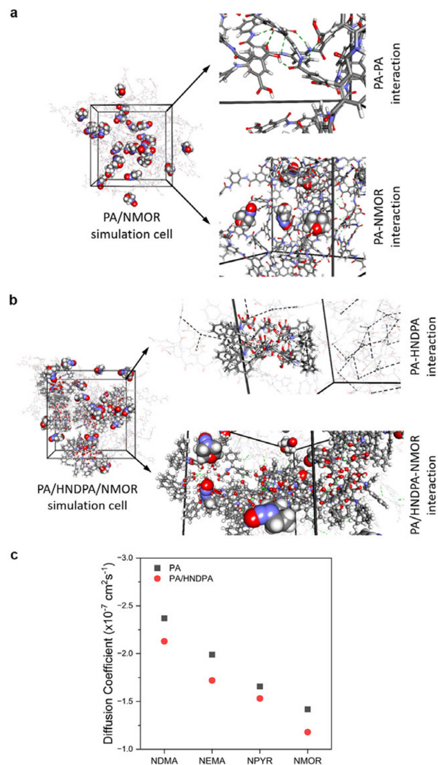
Figure 5. Molecular dynamics analysis of nitrosamine-membrane interactions and transport through polyamide and polyamide/HNDPA systems. (a) Representative MD snapshot of the polyamide–NMOR system, showing hydrogen bonding interactions and spatial confinement of NMOR within the polymer matrix. (b) Corresponding polyamide/HNDPA–NMOR system, showing \pi – \pi stacking alongside hydrogen bonding interactions. (c) Diffusion coefficients of nitrosamine solutes in polyamide and polyamide/HNDPA membranes obtained from MD simulations.
