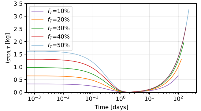
Fig. 3. Evolution of the tritium inventory in the storage for different initial tritium density fractions. The entire transient, up until the doubling time of each scenario, is shown. No reserve inventory is considered.
