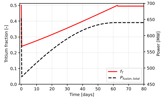
(a) Evolution of tritium density fraction and total fusion power in a tritium-lean scenario with tritium reinjection. Only the initial transient, up until 50:50 DT operation, is shown.
