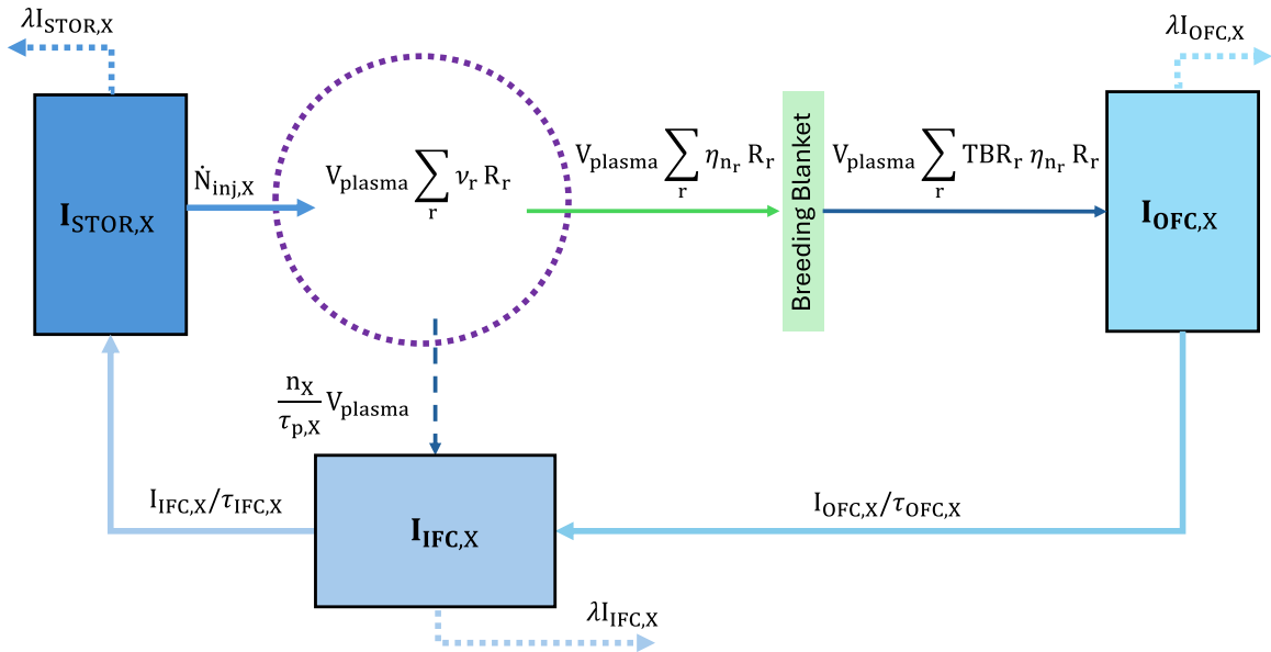
Fig. 2. Diagram of the inventories described by the System of Eqs. (2). Different shades of blue represent a generic species X , green has been used to represent the neutron flux and the breeding blanket (that are not explicitly present in system of equations), while the plasma is represented in purple. The equation representing the plasma have been written using a total number of particles rather than density of species X , to be consistent with the rest of the diagram.
