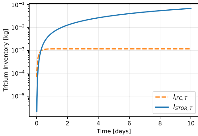
Fig. 5. Evolution of the tritium inventory (IFC and storage) for a 50:50 D 3 He scenario.
