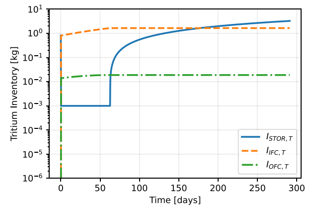
(b) Evolution of tritium inventories in the IFC, OFC and storage in a tritium-lean scenario with tritium reinjection. The entire transient, up until the doubling time, is shown.
