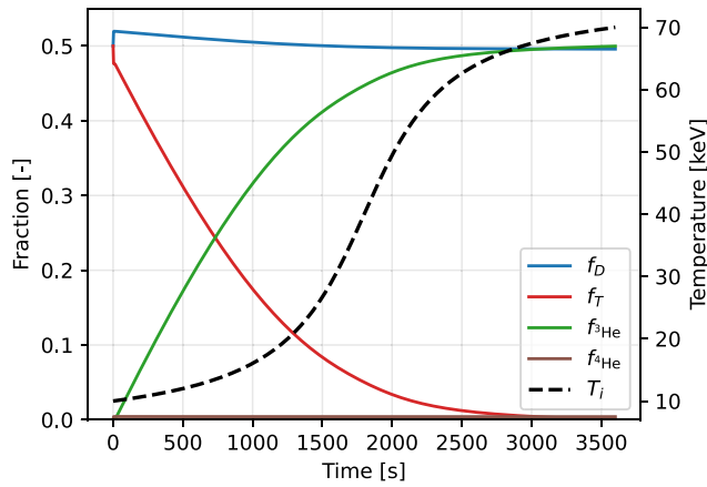
(a) Evolution of each species density fraction and ion temperature in a tritium-assisted D 3 He scenario.
