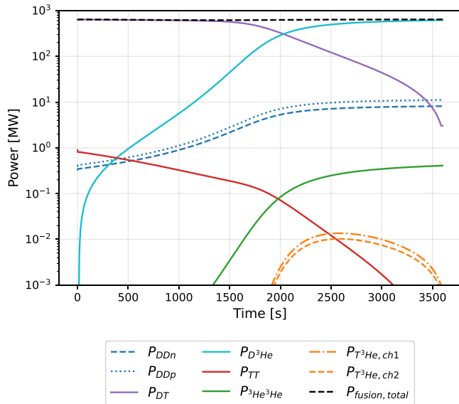
(b) Evolution of each fusion power channel and total fusion power in a tritium-assisted D 3 He scenario.
