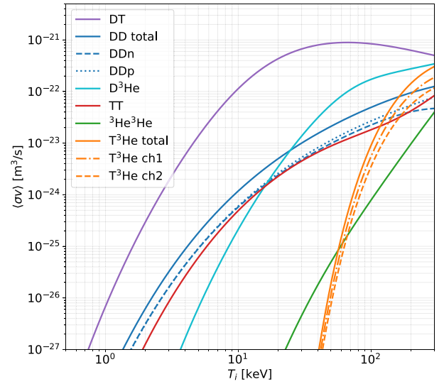
Fig. 1. Nuclear fusion reactivities for the reactions (A)–(H), obtained with analytical formulas [15,17] and used throughout the study.
