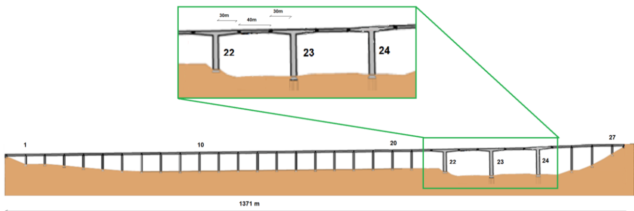
Figure 1: Bridge layout.
