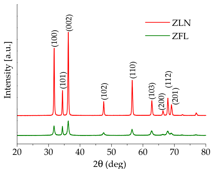
Figure 6. WAXD patterns of needle-like (ZLN) and flower-like nanoparticles (ZFL).
