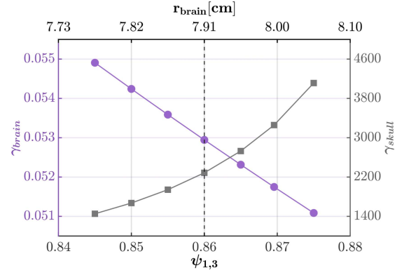
Fig. 4. Polynomial fit of the \gamma parameters for the brain and skull layers as a function of the brain-to-scalp radius ratio \psi_{1,3} . The upper axis also shows the corresponding brain radius r_{\text{brain}} . The skull radius r_{\text{skull}} and scalp radius r_{\text{scalp}} are kept fixed. The dashed vertical line indicates the \gamma values associated with standard brain radius. The curves represent first-order polynomial fit for \gamma_{\text{brain}} ( \text{RMSE} = 2.17 \times 10^{-3} ) and second-order polynomial fit for \gamma_{\text{skull}} ( \text{RMSE} = 1.81 \times 10^{-3} ).
