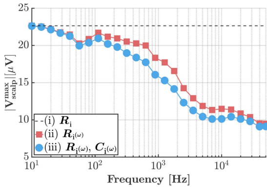
Fig. 8. Frequency response of the maximum scalp potential magnitude |V_{\text{scalp}}^{\text{max}}| predicted by the lumped circuit for a radial dipole at r_{\text{dip}} = 7.40 cm in the three-shell head (cf. Fig. 1). The three cases correspond to: (i) ohmic, nondispersive R_i ; (ii) dispersive R_i(\omega) without displacement currents; and (iii) dispersive R_i(\omega) and dispersive C_i(\omega) .
