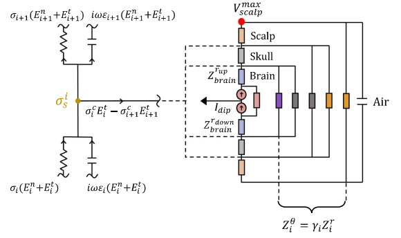
Fig. 2. Lumped-circuit model of a three-layer head with a radially oriented dipolar brain source. Vertically aligned branches implement the radial impedances Z_i^r of each tissue layer; horizontally aligned branches implement the tangential impedances Z_i^\theta . Kirchhoff's current law (KCL) at every node enforces the Neumann boundary condition between adjacent layers i and i+1 , including the effect of the interfacial surface charge density \sigma_s^i that arises from permittivity discontinuities. The brain radial impedances Z_{\text{brain}}^{\text{up}} and Z_{\text{brain}}^{\text{down}} differ according to dipole eccentricity. The source I_{\text{dip}} models the current generated by dipolar neuronal activity and is related to the current dipole moment p_r and the effective dipole length d by I_{\text{dip}} = p_r/d . The point V_{\text{scalp}}^{\max} denotes the maximum scalp voltage.
