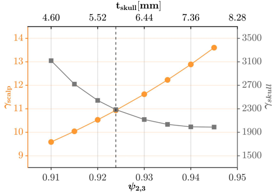
Fig. 5. Polynomial fit of the \gamma parameters for the skull and scalp layers as a function of the skull-to-scalp radius ratio, \psi_{2,3} . The upper axis also shows the corresponding skull thickness t_{\text{skull}} . The brain radius r_{\text{brain}} and scalp radius r_{\text{scalp}} are kept fixed. The dashed vertical line indicates the \gamma values associated with standard skull thickness. The curves represent first-order polynomial fit for \gamma_{\text{scalp}} (RMSE = 5.39 \times 10^{-3} ) and second-order polynomial fit for \gamma_{\text{skull}} (RMSE = 4.81 \times 10^{-3} ).
