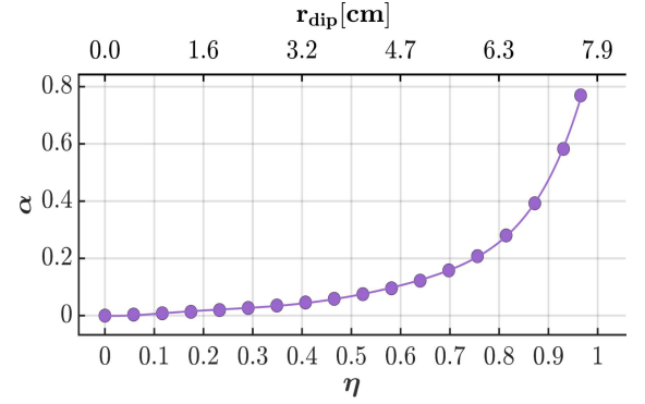
Fig. 3. Polynomial fit of the \alpha parameter as a function of dipole eccentricity, \eta (bottom axis) and dipole radius, r_{\text{dip}} (upper axis). The best-fit curve is a six-order polynomial ( \text{RMSE} = 2.33 \times 10^{-3} ).
