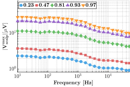
Fig. 6. Frequency-domain comparison of the maximum scalp potential magnitude predicted by the semi-analytical model (solid lines) and the lumped RC circuit (dashed lines) for different dipole eccentricities.
