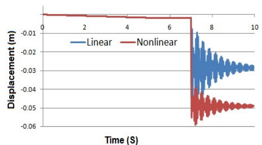
Figure 8. Displacement time history of case 2
