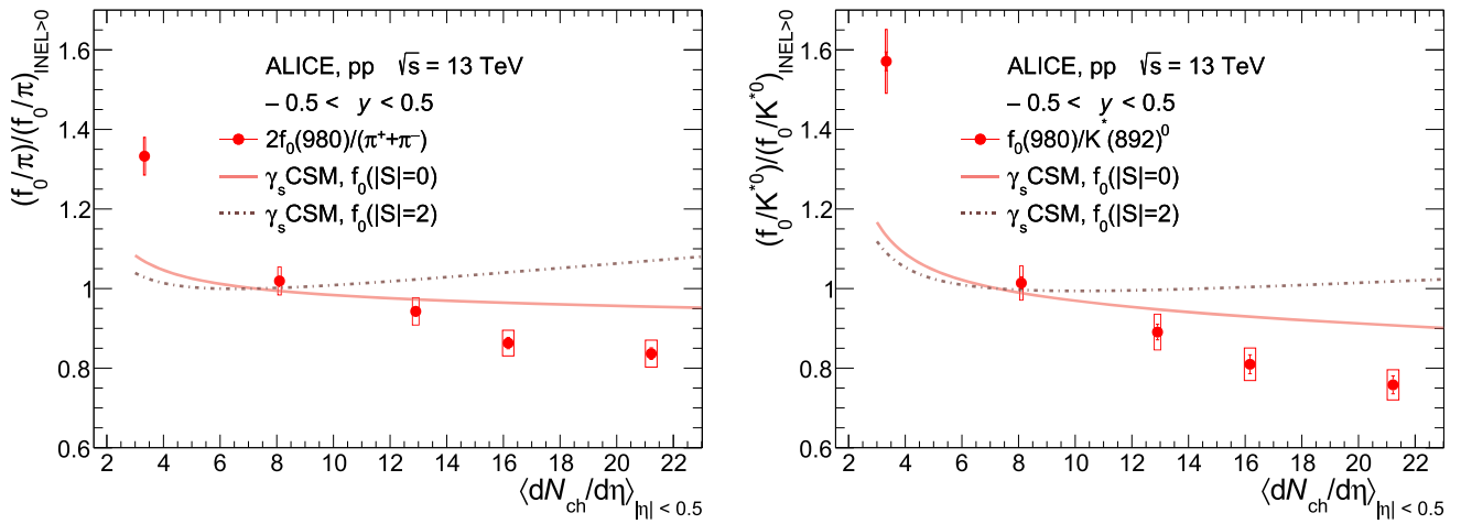
Fig. 6 Double ratios of f_0(980) to \pi (left panel) and K^*(892)^0 (right panel) as a function of charged-particle multiplicity. The single ratio is divided by the ratio in INEL > 0 events, which cancels correlated sys-
