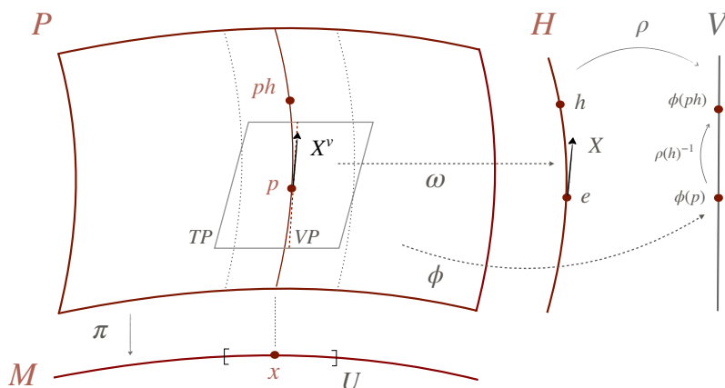
Fig. 1 Schematic visualization of the principal bundle P , with structure group H , a vertical vector X^v , a (principal) connection \omega , and tensorial 0-form (matter field) \phi
