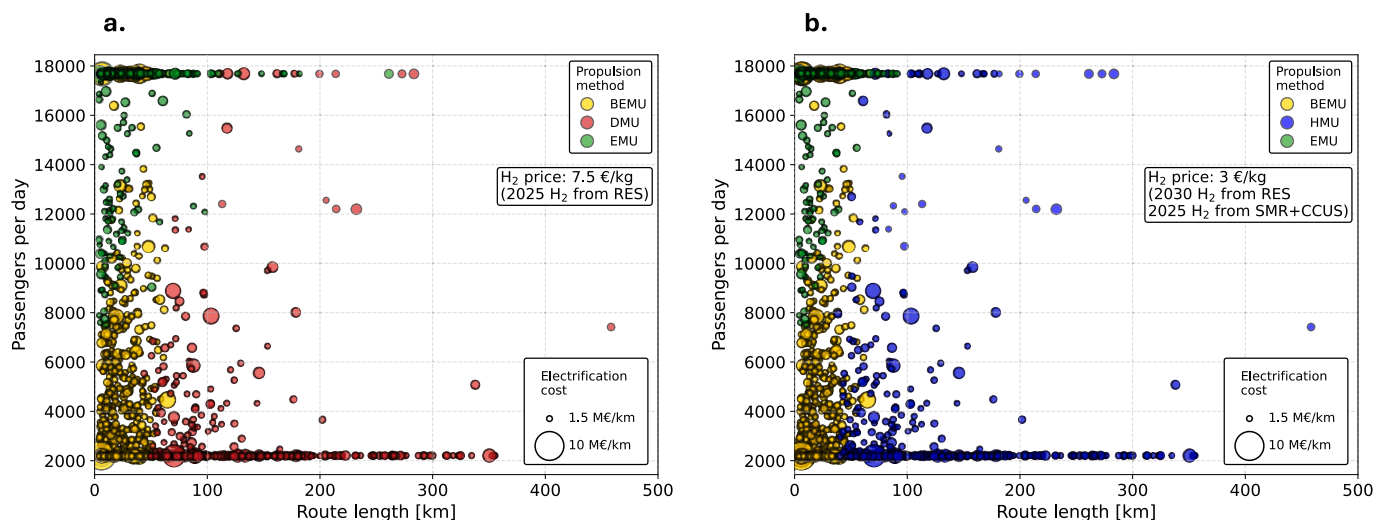
Fig. 4. Bubble plot of non-electrified European railway lines: a. €7.5/kg H 2 price (current price of electrolysis from RES); b. €3/kg H 2 price (current price of SMR + CCS and 2030 price of electrolysis from RES). The size of each bubble is proportional to the specific electrification cost of the line (M€/km).
