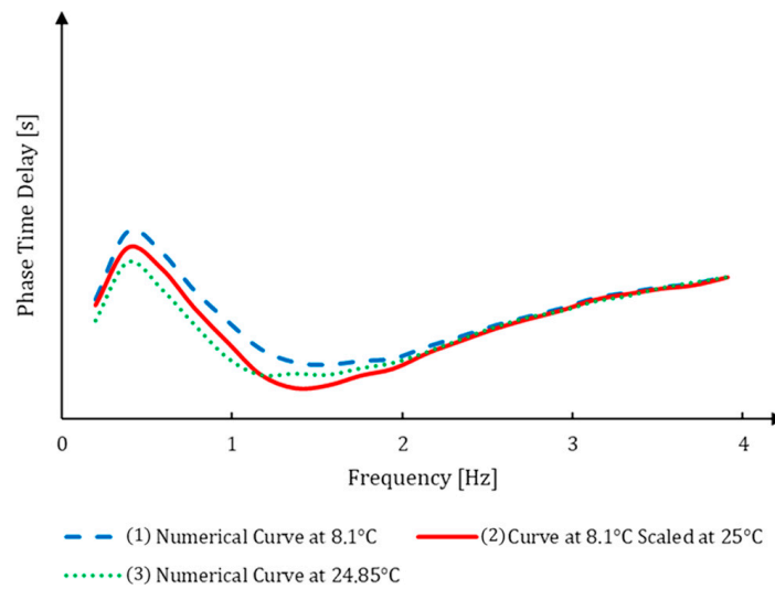
Figure 12. G'_3 (= \beta / \delta_{sw}) , gain, phase and phase time delay, numerical results comparison.
