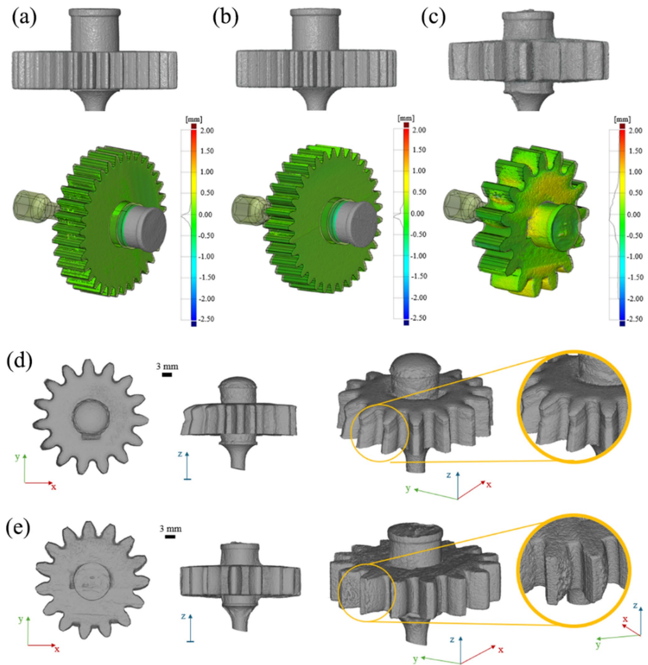
Fig. 7 Ct scan images. (a–c) Comparison with the CAD model: (a) Sample H1_8 , virgin powder; (b) sample V1_8 , virgin powder; (c) sample V2_{10\_g} , refreshed powder, approximately 86 h. (d) Sample H2_{10\_g} , (e) sample V2_{10\_g}
