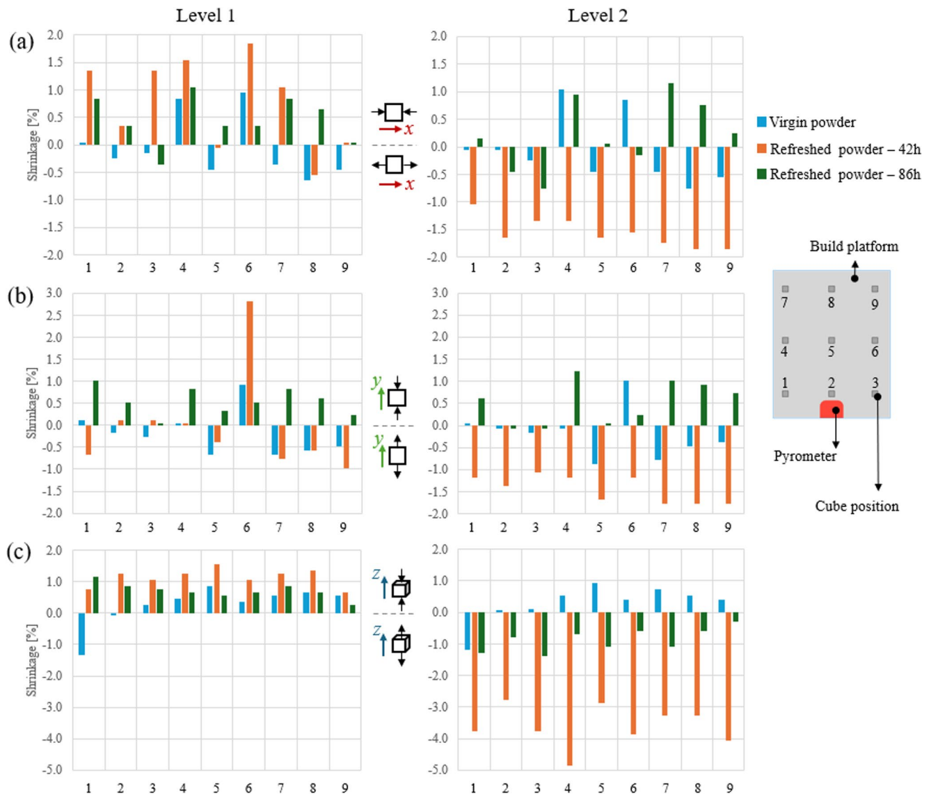
Fig. 8 Position of the cubes and their relative shrinkage with respect to the three Cartesian coordinates
