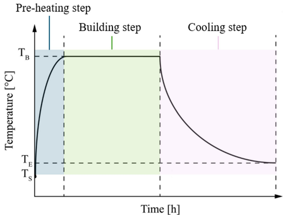
Fig. 1 Schematic representation of a temperature profile of PBF-LB/P process. T_s is starting temperature
