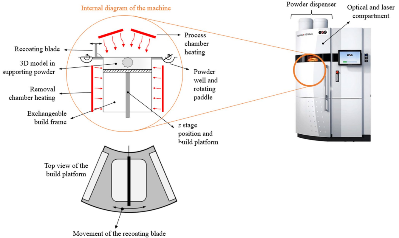
Fig. 5 Schematic representation of the EOS Formiga P110 Velocis
