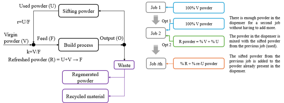
Fig. 2 Schematic sequence of powder usage in jobs. U, V, F and O represent the used powder, virgin powder, feed and outlet streams, respectively. The fraction of used and virgin material (refreshed powder) is defined by the ratios r=U/F and k=V/F , related via the material balance, F=U+V
