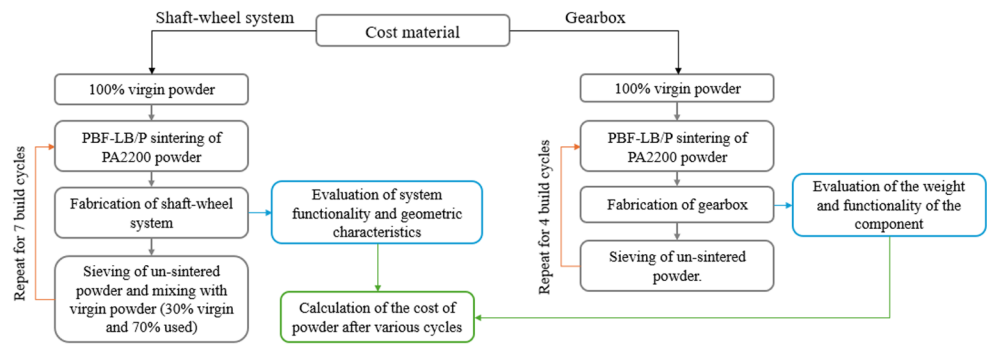
Fig. 4 Data creation flowchart for cost material validation
