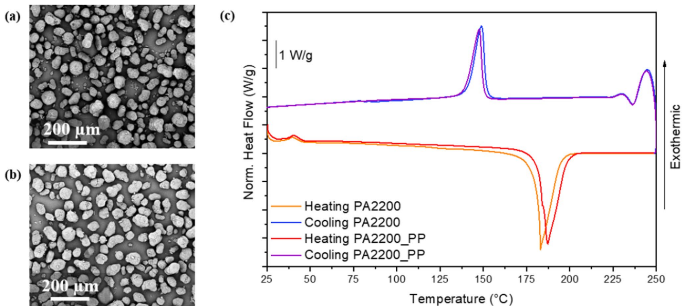
Fig. 6 (a) Virgin, (b) recycled powder, (c) DSC plot of the virgin and recycled powder
