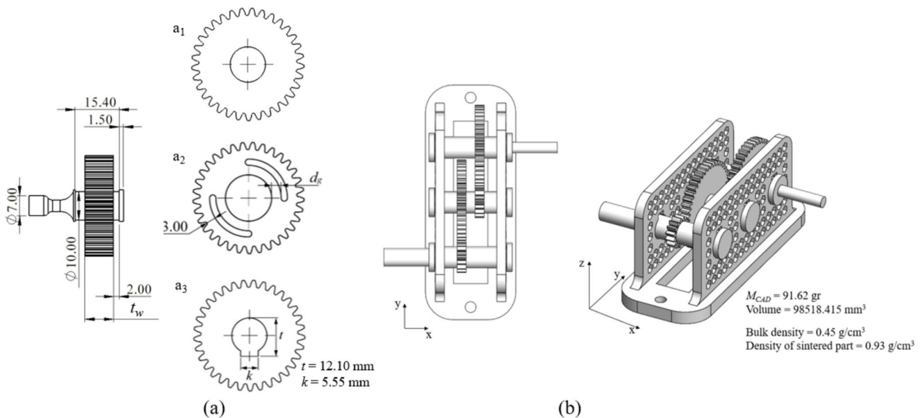
Fig. 3 Integrated mechanical gear design. (a) Shaft-wheel system with different wheel designs: (a 1 ) with standard geometry, (a 2 ) with slots, (a 3 ) with a groove between wheel and shaft. (b) Gearbox
