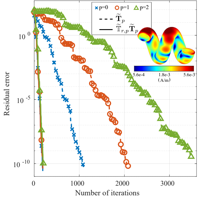
Fig. 4. Residual error of the iterates as a function of the number of iterations of TFQMR and surface current density (in A/m) obtained for p = 2 .
