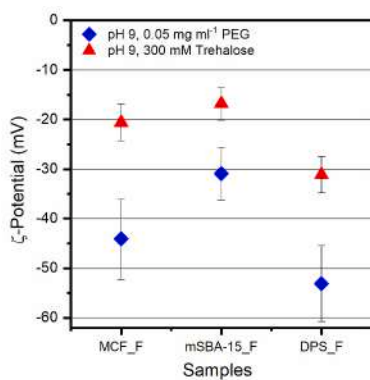
Fig. 9. ζ-potential measured for functionalized MCF, mSBA-15, and DPS suspended in 25 mM carbonate buffer pH 9 with 0.05 mg mL -1 PEG (◆) or 300 mM trehalose (▲). 55.
