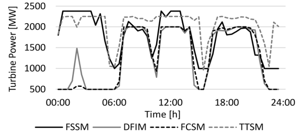
Fig. 7 Median half-hourly turbine power level with different PHSP schemes.
