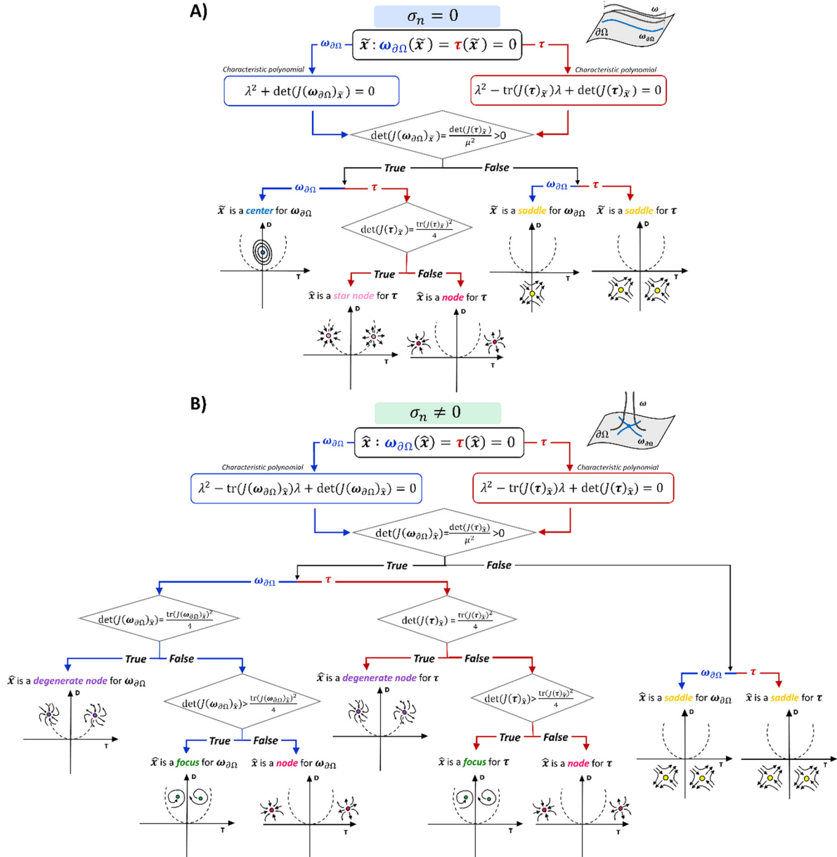
FIG. 3. Chart of the analysis of wall shear stress and surface vorticity fixed points in the case of (A) null vorticity diffusion flux normal to the wall and (B) not-null vorticity diffusion flux normal to the wall.
