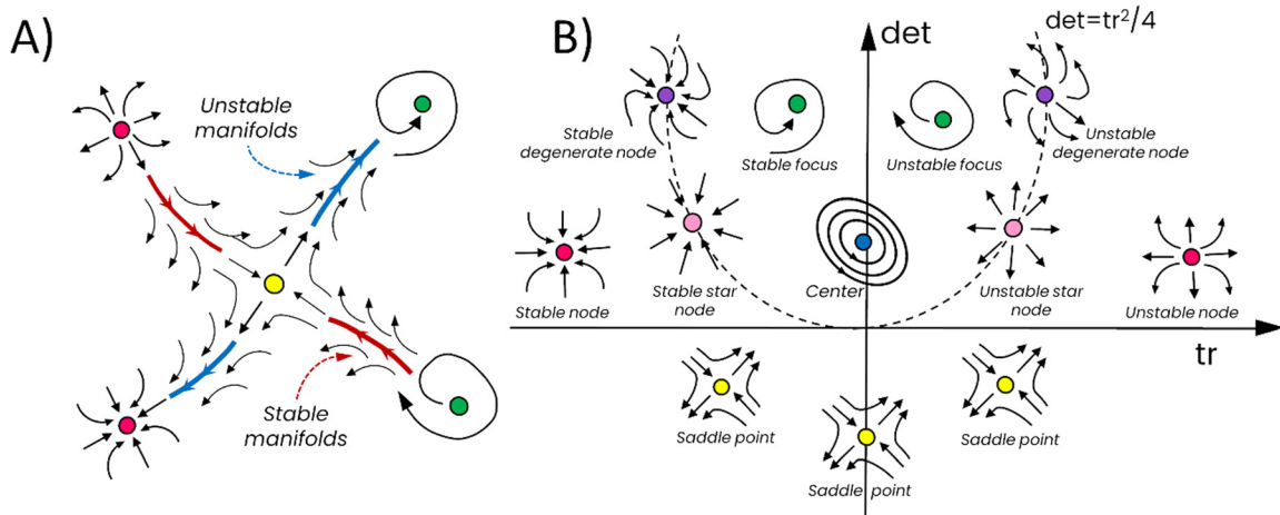
FIG. 2. (A) Explanatory sketch of the stable/unstable manifold configurations linking fixed points; (B) stability and type of fixed points of a vector field in the \text{tr} - \text{det} plane, where \text{tr} and \text{det} refer to the trace and determinant of the Jacobian matrix of the vector field respectively. The dotted line represents the critical quadratic curve splitting the \text{det} > 0 region in two subregions where the eigenvalues of the Jacobian matrix of the vector field are complex or real numbers. Inspired by Perry and Fairlie. 54
