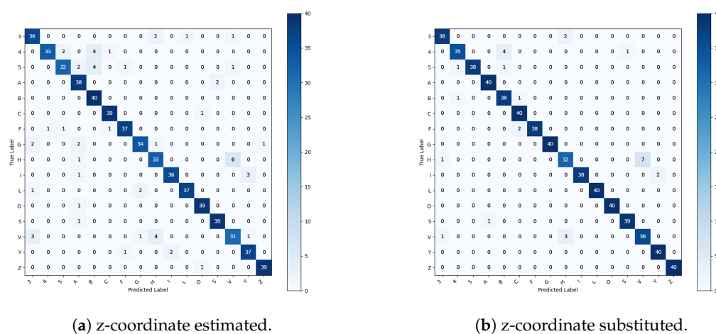
Figure 10. Confusion matrices referring to the datasets representing the sixteen configurations.
