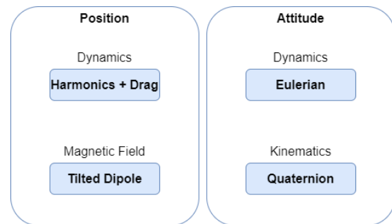
Figure 2: Plant Modeling
