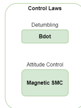
Figure 4: Implemented Control Laws
