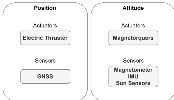
Figure 5: Implemented Hardware
