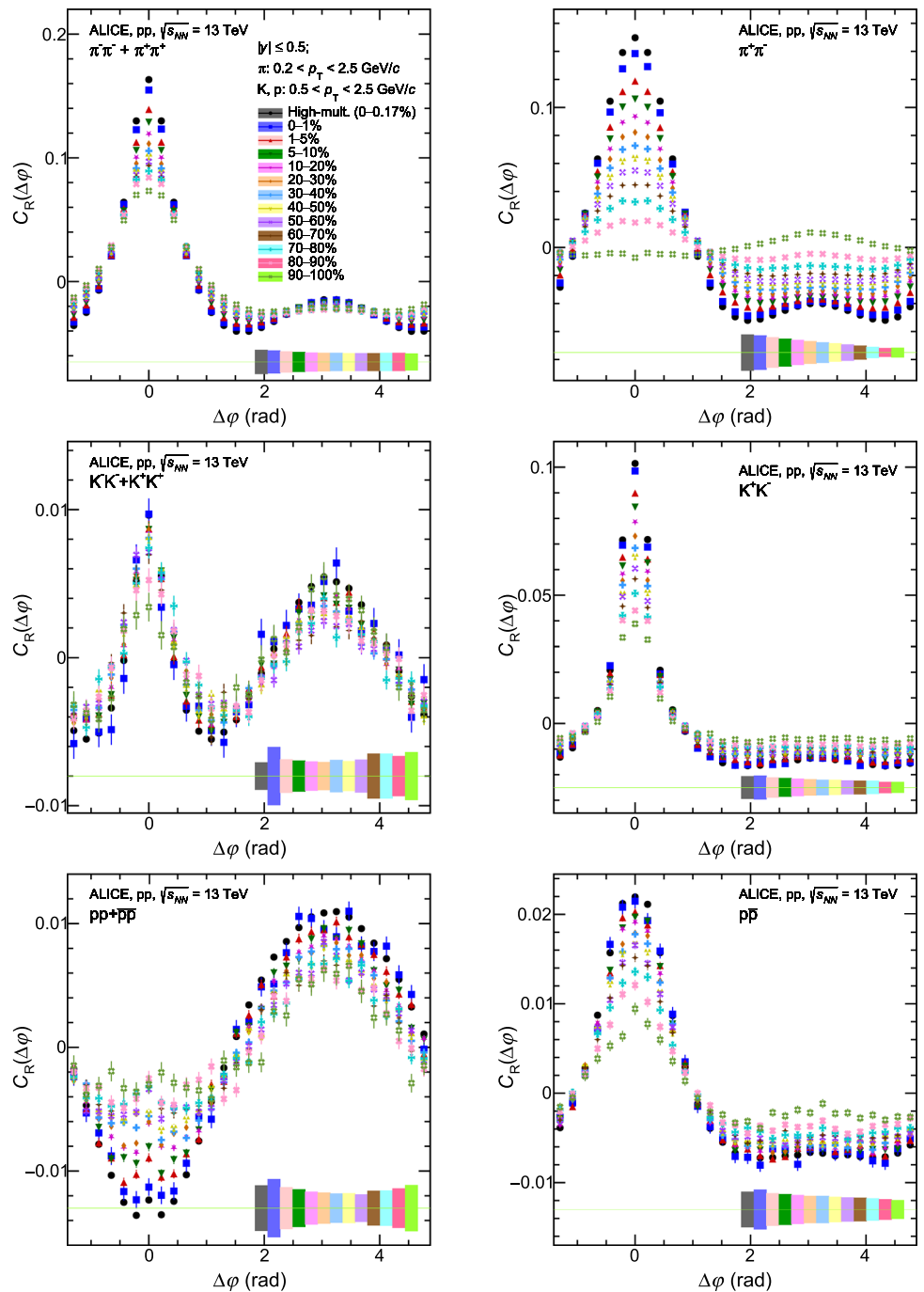
Fig. 4 \Delta\phi projections of correlation functions within |\Delta y| < 1 for like- and unlike-sign pions, kaons, and protons in multiplicity classes, using the C_R definition. Statistical uncertainties (bars) and systematic uncertainties (boxes) are both drawn with the colour associated with the corresponding multiplicity class.
