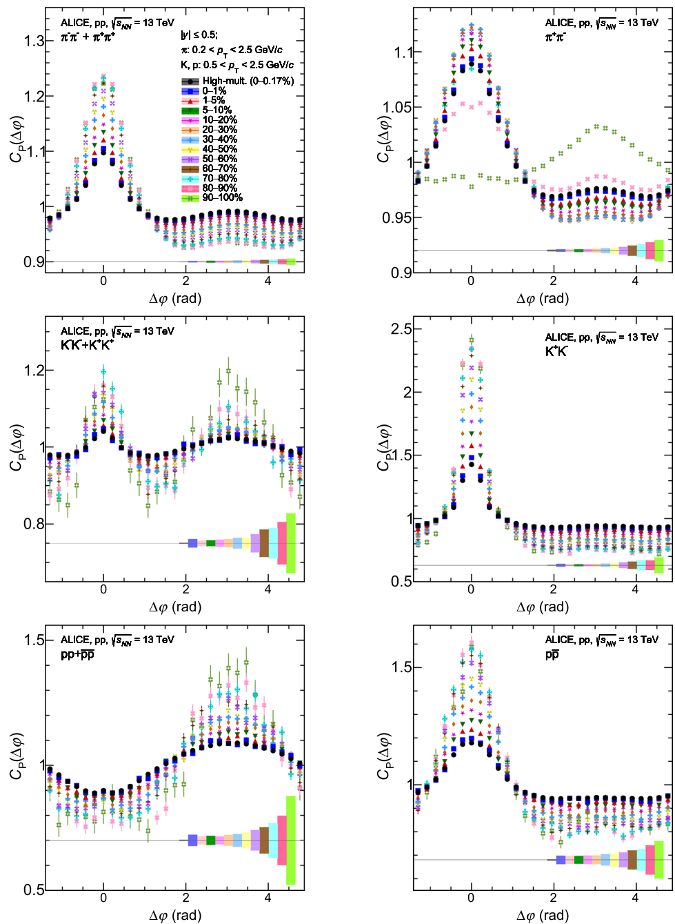
Fig. 3 \Delta\phi projections of correlation functions within |\Delta y| < 1 for like- and unlike-sign pions, kaons, and protons in multiplicity classes, using the C_P definition. Statistical uncertainties (bars) and systematic uncertainties (boxes) are both drawn with the color associated with the corresponding multiplicity class.
