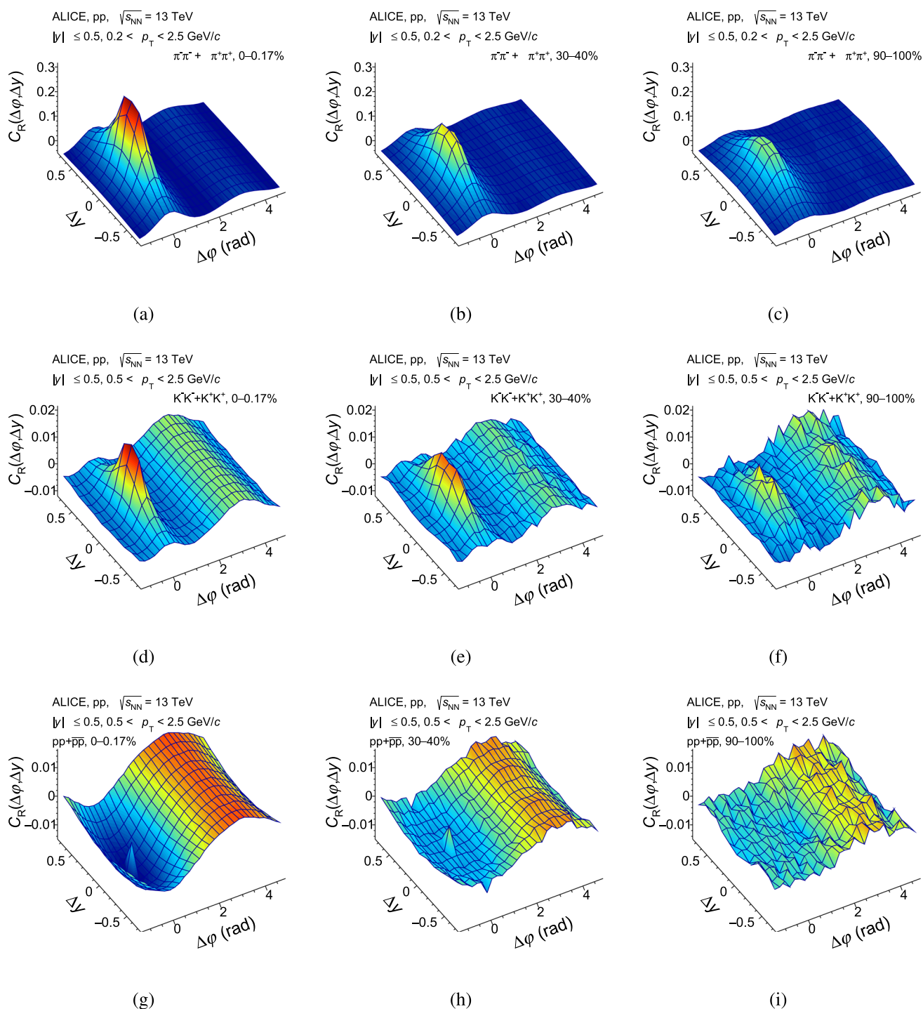
Fig. 1 The (\Delta y, \Delta\phi) correlation functions for like-sign pions, kaons, and protons pairs (top-to-bottom) in the highest (0–0.17%), the middle (30–40%), and lowest (90–100%) multiplicity classes (left-to-right) of pp collisions at \sqrt{s} = 13 TeV using the C_R definition.
