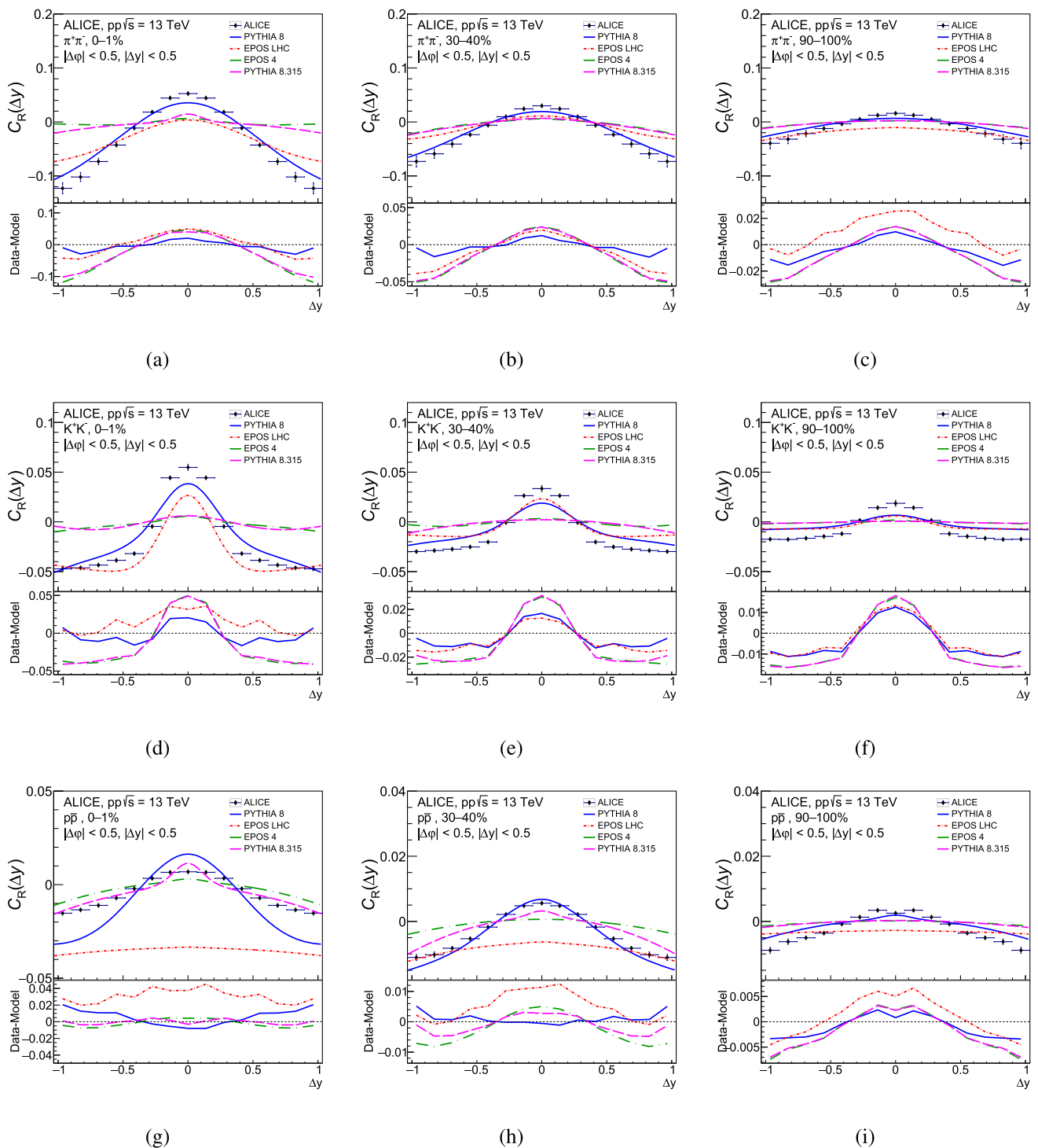
Fig. 8 \Delta y -correlation function distribution compared with MC models (PYTHIA8 Monash 2013 in blue, EPOS LHC in red, EPOS4 in green, and PYTHIA 8.315 in magenta) in pp collision at \sqrt{s} = 13 TeV
