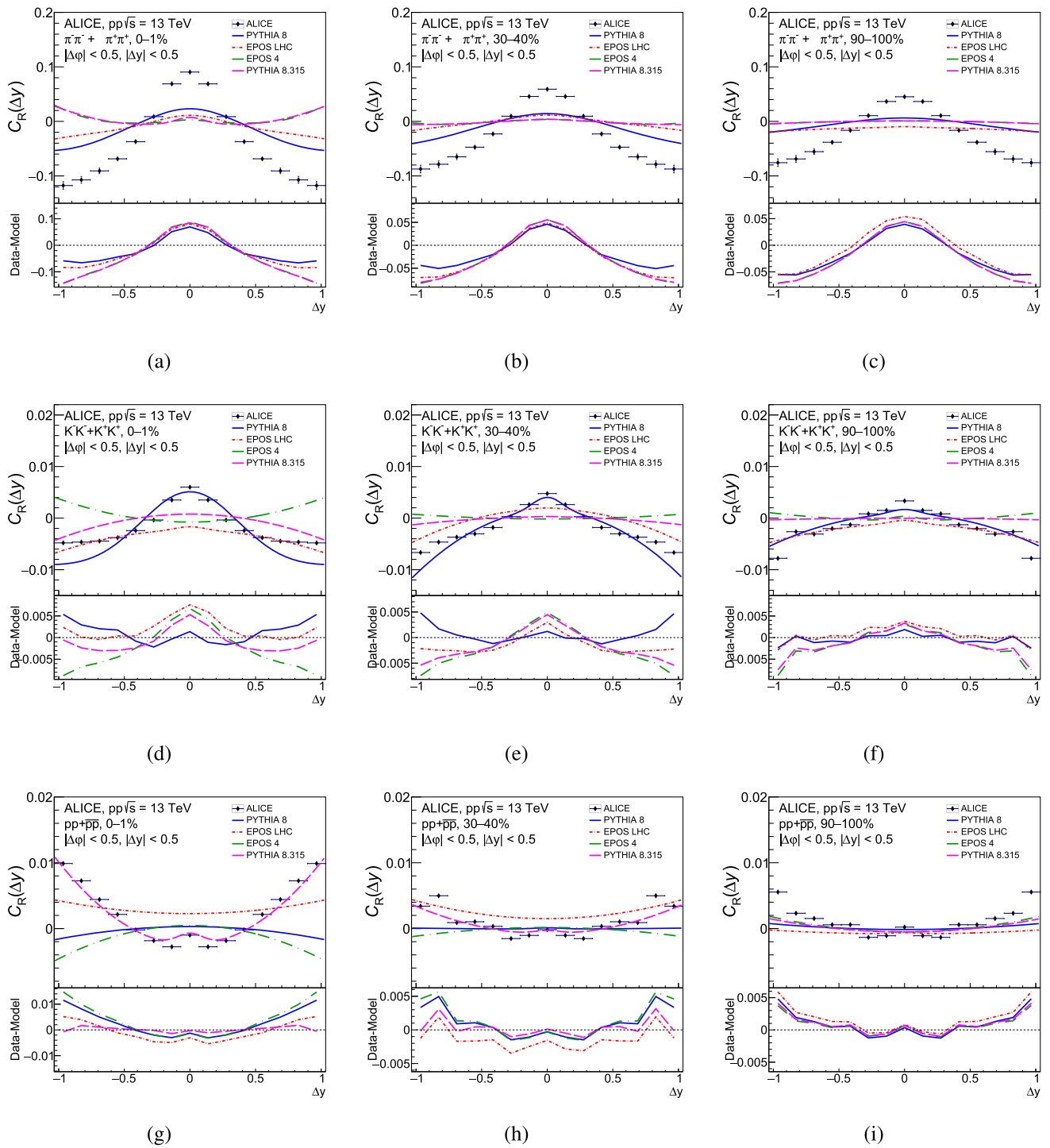
Fig. 7 \Delta y -correlation function distribution compared with MC models (PYTHIA8 Monash 2013 in blue, EPOS LHC in red, EPOS4 in green, and PYTHIA 8.315 in magenta) in pp collision at \sqrt{s} = 13 TeV
