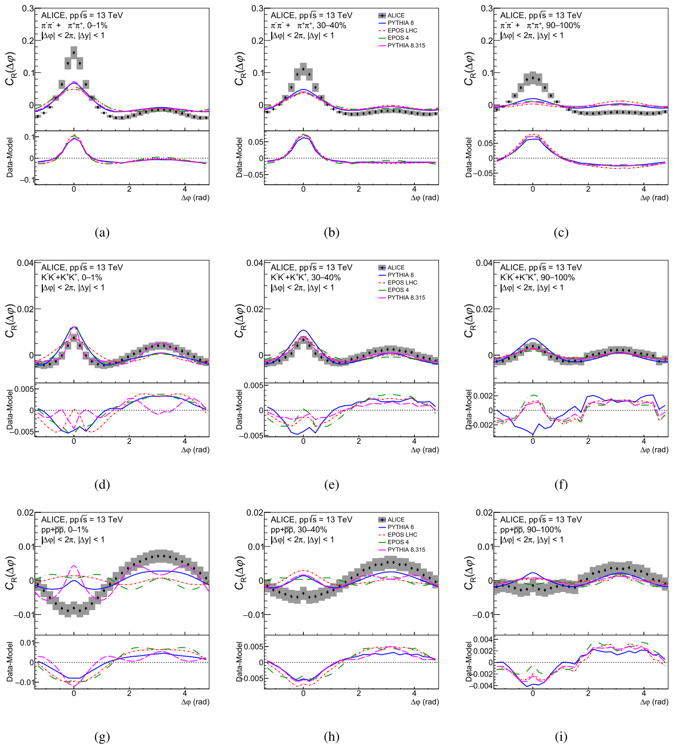
Fig. 5 Comparison between \Delta\phi -correlation functions and MC models (PYTHIA8 Monash 2013 in blue, EPOS LHC in red, EPOS4 in green, and PYTHIA 8.315 in magenta) in pp collision at \sqrt{s} = 13 TeV by
