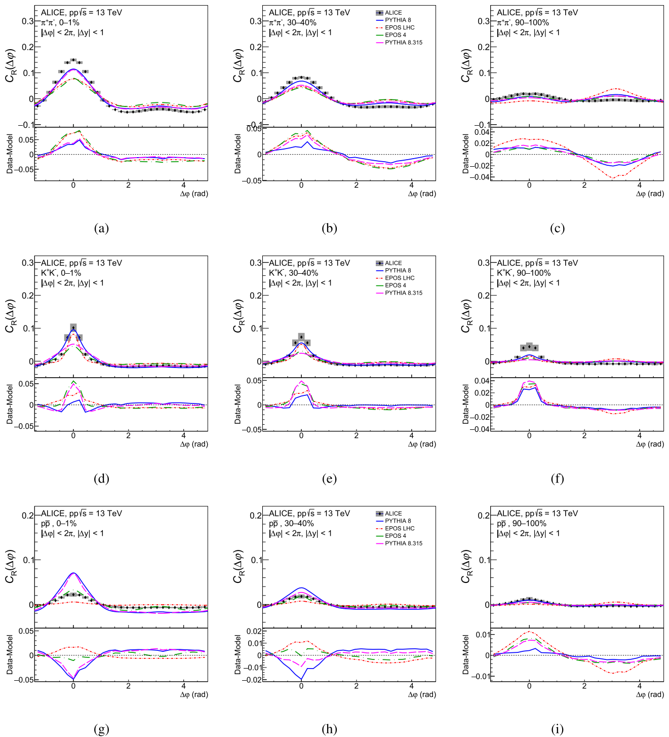
Fig. 6 Comparison between \Delta\phi -correlation functions and MC models (PYTHIA8 Monash 2013 in blue, EPOS LHC in red, EPOS4 in green, and PYTHIA 8.315 in magenta) in pp collision at \sqrt{s} = 13 TeV
