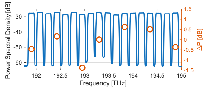
Fig. 10. Transmit optical spectrum with unequal power among the WDM channels (blue line, left axis). The power difference with respect to the central WDM channel is highlighted by the red circles (right axis).
