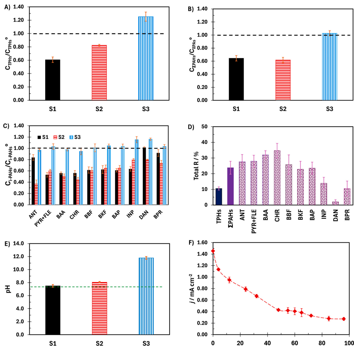
Fig. 1. Effect of the electrochemical remediation of real marine sediments of Bagnoli Bay under 0.25 \text{ V cm}^{-1} on the normalized concentration of (A) TPHs, (B) ΣPAHs, and (C) each detected PAH (ANT, FLE + PYR, BAA, CHR, BBF, BKF, BAP, INP, DAN, BPR) in the region S1, S2 and S3 after 96 h. (D) Total removal of TPHs, ΣPAHs, ANT, FLE + PYR, BAA, CHR, BBF, BKF, BAP, INP, DAN and BPR from the sediment. (E) Plot of the pH in the region S1, S2 and S3 after 96 h. (F) Plot of current density ( j ) vs. time during the ER treatment. Error bars indicate the standard deviation calculated from two independent experiments. The dashed black line in the Figures A, B and C represents the zero time where the C_i/C_i^0 ratio is \sim 1 . The dashed green line in the Figure E represents the pH at the zero time.
