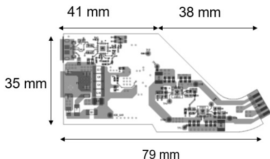
Fig. 4: Radar power supply board final form (Top Layer)
