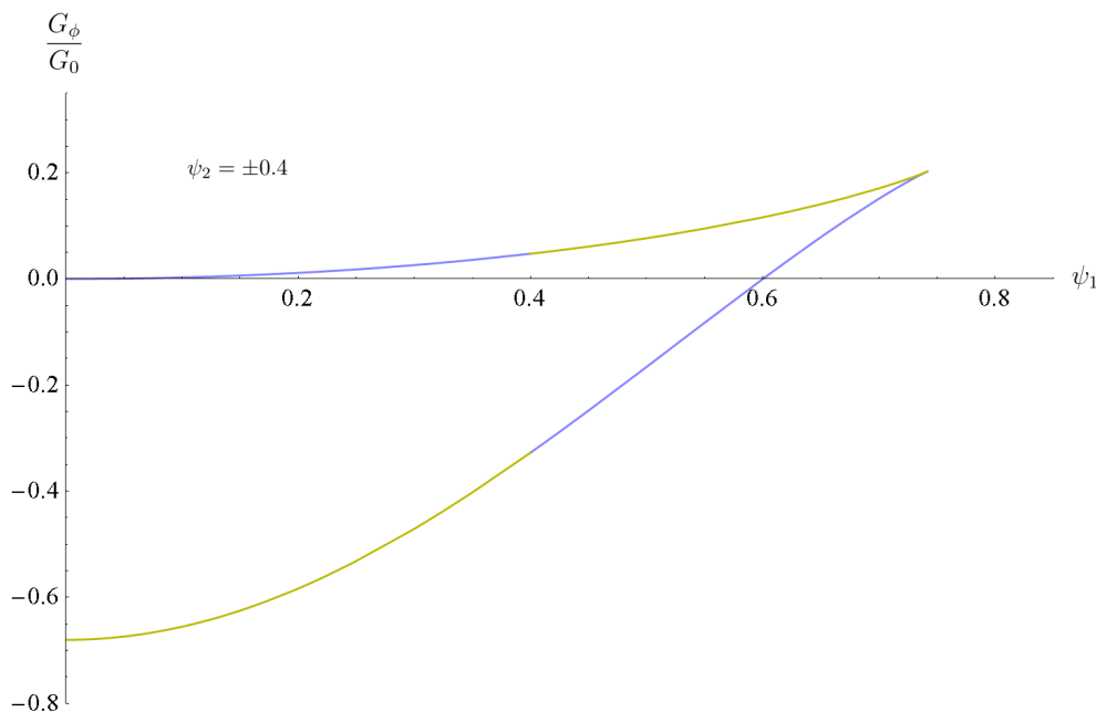
Figure 3. Rescaled free energy \frac{G_\phi}{G_0} as a function of \psi_1 , for \psi_2 = \pm 0.4 . The x \gtrless 1 branches of the solution are represented by different hues. The shift in color occurs when one of the spacetimes, pertaining to a configuration, transits into another (see section 4).
