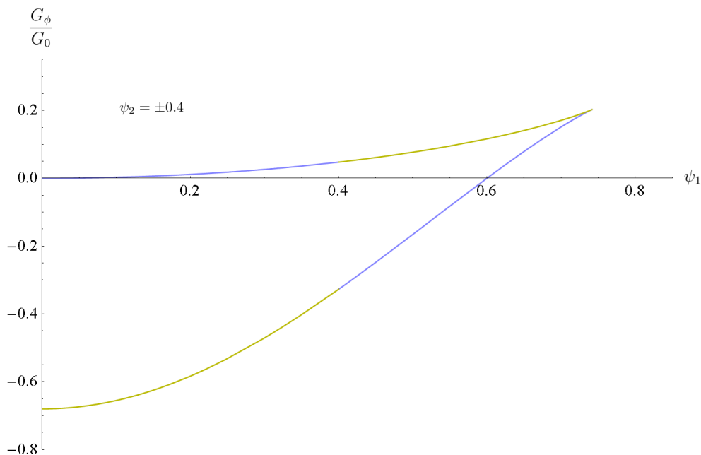
Figure 3. Rescaled free energy \frac{G_\phi}{|G_0|} as a function of \psi_1 , for \psi_2 = \pm 0.4 . The x \gtrless 1 branches of the solution are represented by different hues. The shift in color occurs when one of the spacetimes, pertaining to a configuration, transits into another (see section 4).
