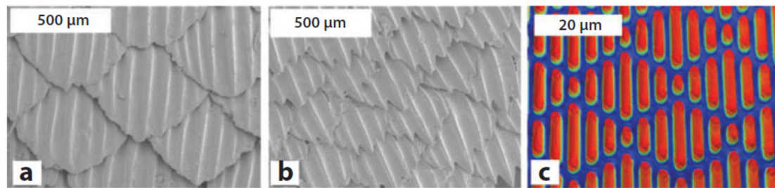
Figure 6. SEM micrographs of (a) spinner shark skin and (b) Galapagos shark skin surfaces. (c) Optical profilometry of sharklet surface. Reprinted with permission [127] © 2010 Elsevier.
