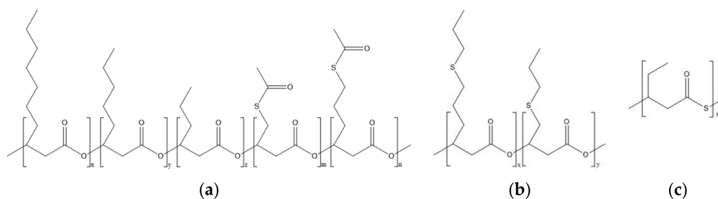
Figure 5. Chemical structure of polyhydroxyalkanoates (PHAs) containing sulfur. (a) PHAs with thioester linkages in their side chains (PHACOS). (b) PHAs with thioether linkages in their side chains (poly(3HPTB-co-3HPTHx)). (c) PHAs with thioester groups in their main chains (poly(3MV)).
