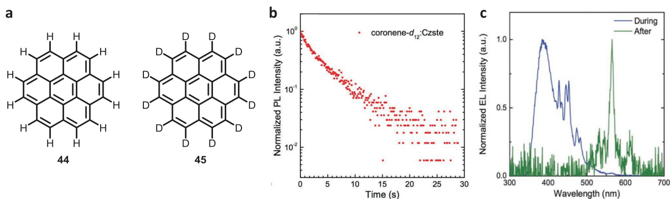
Figure 13. a) Chemical structures of coronene ( 44 ) and coronene- d_{12} ( 45 ). b) Transient PL intensity of 45 @CzSte at 560 nm. c) Electroluminescence spectra of 45 @CzSte during and after electrical excitation (blue and green lines, respectively). Reproduced with permission. [120] Copyright 2016, Wiley-VCH.
