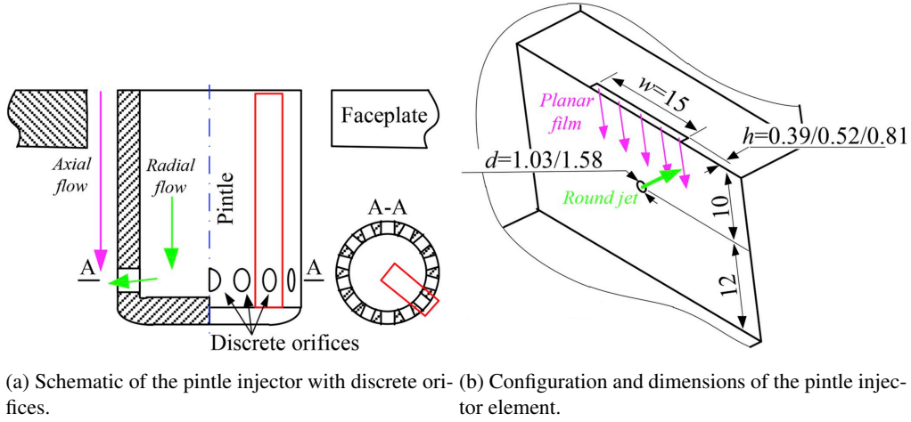
Figure 4: Testcase pintle injector [10] .
