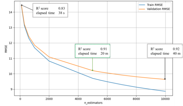
Fig. 3. XGB performances
