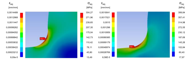
Figure 13 Calculated maximum equivalent stress \sigma_{eq} and strain values \epsilon_{eq} and position (left side for standard gear and right side for thin-rim gear).
