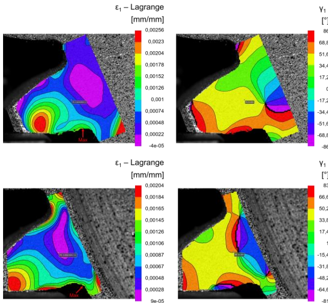
Figure 14 Experimental maximum principal strain \epsilon_1 and maximum principal direction \gamma_1 maps for standard (upper) and thin-rim (lower) gears.
