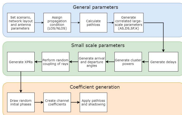
FIGURE 3. Channel coefficient generation in 3GPP 3D channel model.
