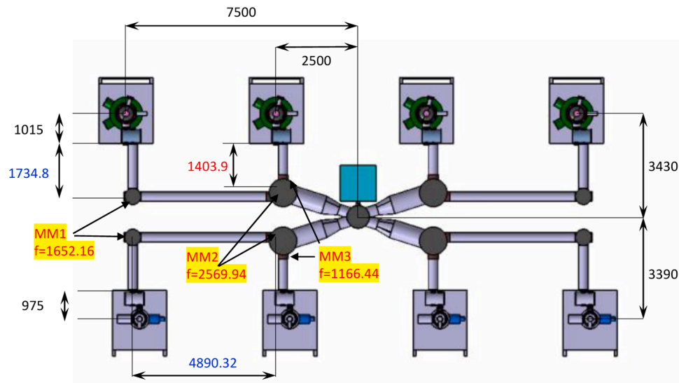
Fig. 4. Distances and focal lengths chosen for the single-beam transmission lines (in mm units).
