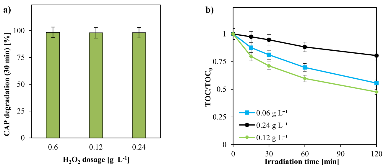
Fig. 9. (a) CAP degradation efficiency after 30 min of dark-phase treatment using Fe^0(3.3\%)/Fe_3O_4(1.6\%)/USY\ 360 at different H 2 O 2 dosages; (b) CAP mineralization under solar irradiation (expressed as the ratio TOC/TOC 0 , where TOC is the residual total organic carbon at time t, and TOC 0 is the initial value) as a function of irradiation time at different H 2 O 2 dosages. Reaction conditions: [CAP]_0 = 25 ppm, pH = 4, catalyst dosage = 1.5 g L -1 .
