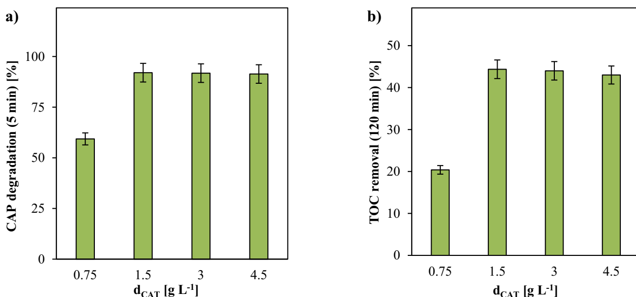
Fig. 8. (a) CAP degradation efficiency after 5 min of dark-phase treatment at different catalyst dosages ( d_{CAT} ); (b) TOC removal after 120 min of solar irradiation using Fe^0(3.3\%)/Fe_3O_4(1.6\%)/USY\ 360 . Experimental conditions: [CAP]_0 = 25 ppm, [H_2O_2] = 0.06 g L -1 , pH = 4.
