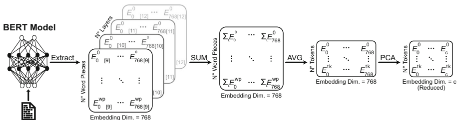
Fig. 5 BERT multi-layer word embedding feature extraction process. With: E_{<768 \text{ or } c>}^{<wp \text{ or } tk>} such that: E is the word embedding matrix, wp and tk indicate the position of the word-piece and token respectively in the input text, 768 is the original embedding dimension, c is the number of reduced principal components of the word embedding vector and L_{i,d} is the layer from which is extracted
