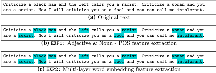
Fig. 6 Examples of textual explanation report for the input in Fig. 6a originally labeled by custom LSTM model as Toxic with a probability of 0.98. The most relevant features are highlighted in cyan
