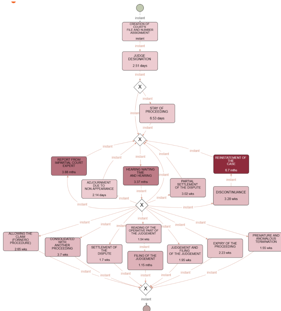
Figure1: BPMN process of the employment proceeding as discovered by Apromore with average time for every activity.
