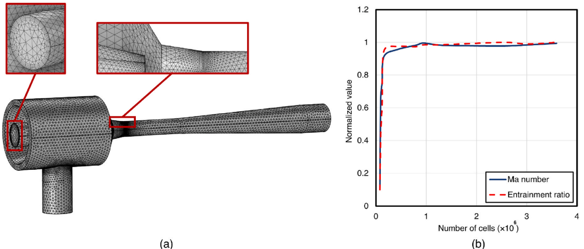
Fig. 3. Representation of (a) computational domain and grid structure of the ejector, and (b) grid independence study considering the magnitudes of both Ma and \omega
