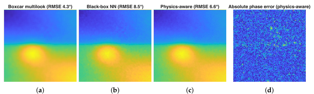
Figure 8. Representative reconstructions for the illustrative InSAR case study. In the shown scene, the classical boxcar multilook baseline remains strongest, while the physics-aware estimator improves over the black-box neural network but does not surpass the phase-preserving baseline. Colors follow the MATLAB parula colormap, with dark blue indicating lower estimated phase values and yellow indicating higher values.
