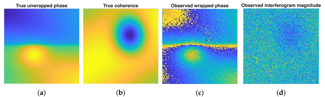
Figure 7. Observation-side quantities for the illustrative InSAR phase-domain case study. The synthetic example includes a smoothly varying unwrapped phase field, a nonuniform coherence map, the corresponding wrapped phase observation, and the observed interferogram magnitude. Colors follow the MATLAB parula colormap, where dark blue corresponds to lower phase values and yellow to higher phase values in the phase panels.
