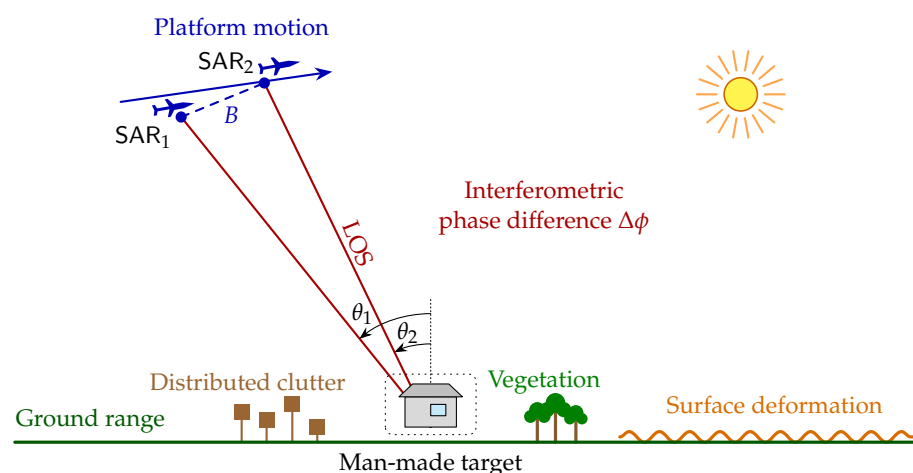
Figure 2. Illustrative SAR/InSAR sensing scenario. Two radar acquisitions with baseline B observe a scene containing a man-made target (stylized house in a dotted box), distributed clutter, vegetation, and a deforming surface patch. The geometry highlights the line of sight, the incidence angles \theta_1 and \theta_2 , and the interferometric phase difference \Delta\phi . The presence of sunlight recalls that, unlike optical sensing, radar acquisition is independent of solar illumination.
