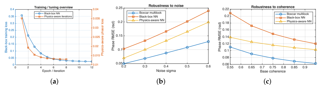
Figure 9. Optimization and robustness summaries for the illustrative InSAR phase-domain case study. The black-box loss decreases during training, the physics-aware phasor loss decreases across iterations, and both learned approaches degrade as observation quality worsens.
