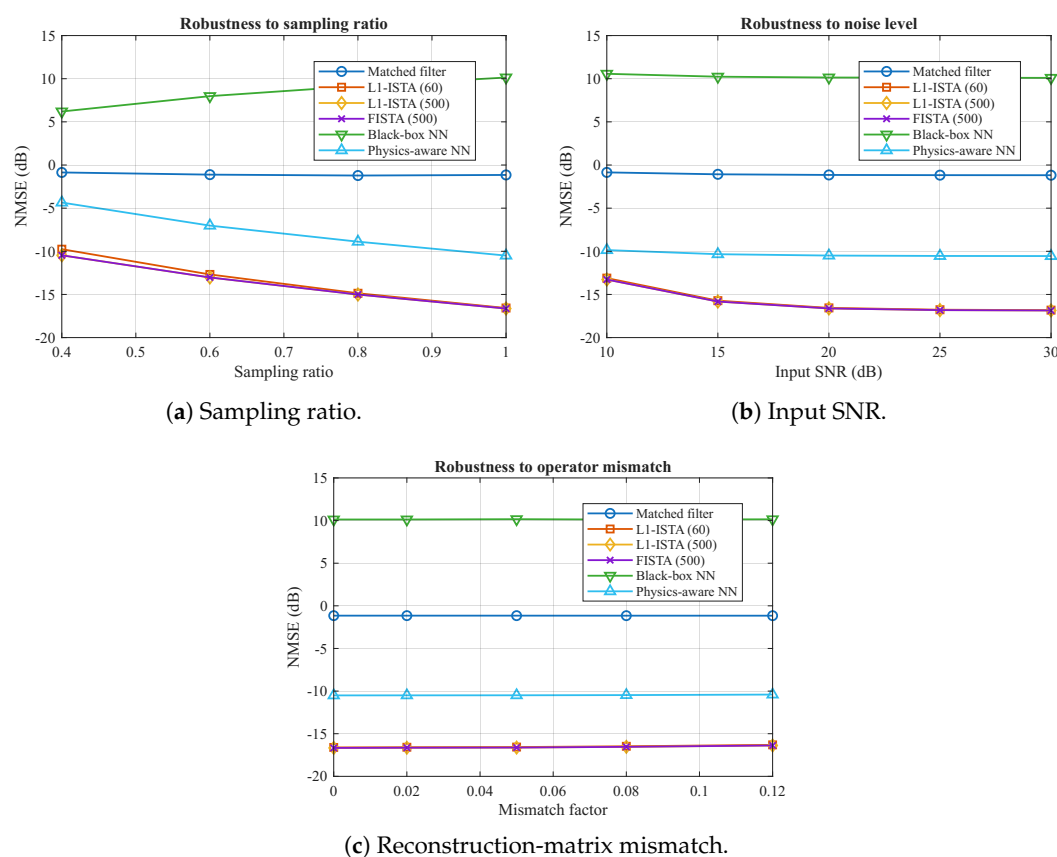
Figure 6. Robustness analysis for the constructive sparse SAR experiment. Each panel includes the matched filter, finite-depth \ell_1 -ISTA, long-run \ell_1 -ISTA, long-run FISTA, black-box NN, and physics-aware NN, with the legend identifying the line style used for each method. The stronger classical baselines provide the lowest NMSE, while the learned physics-aware model should be interpreted as a fixed-depth reconstruction strategy.
