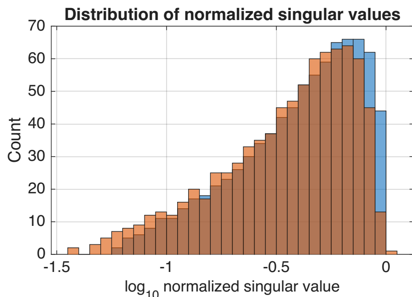
Figure 3. Histogram of normalized singular values for the explicit SAR sensing matrix (orange), compared with a complex Gaussian reference matrix of the same dimensions with i.i.d. entries distributed as \mathcal{CN}(0, 1/N) (blue), with some overlap between the two distributions (brown). A larger fraction of the normalized singular values lies near zero for the SAR matrix than for the Gaussian reference, which indicates stronger deterministic structure, higher coherence, and poorer conditioning. The Gaussian matrix is included as a diagnostic benchmark for matrix structure and is not used as a forward model in the reconstruction experiment.
