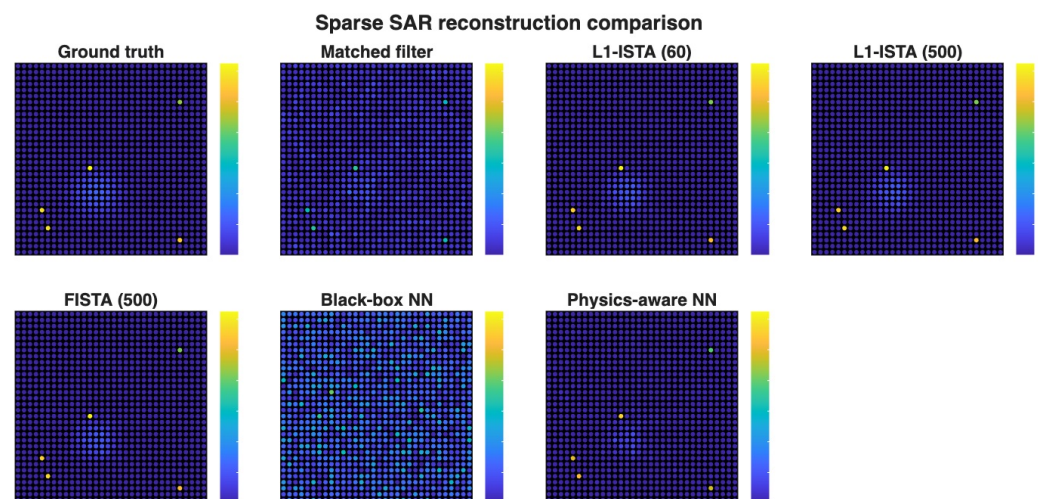
Figure 4. Sparse SAR reconstruction comparison on a representative synthetic scene. All panels display the normalized magnitude |x|/\max|x_{\text{true}}| using a common color scale, with dark colors corresponding to values near 0 and bright yellow corresponding to values near 1. In addition to the finite-depth \ell_1 -ISTA baseline, long-run \ell_1 -ISTA and FISTA are included as stronger classical optimization references. The results show that fully converged iterative solvers remain highly competitive in NMSE, while the physics-aware network should be interpreted as a fixed-depth model-guided reconstruction strategy rather than as a replacement for converged variational optimization.
