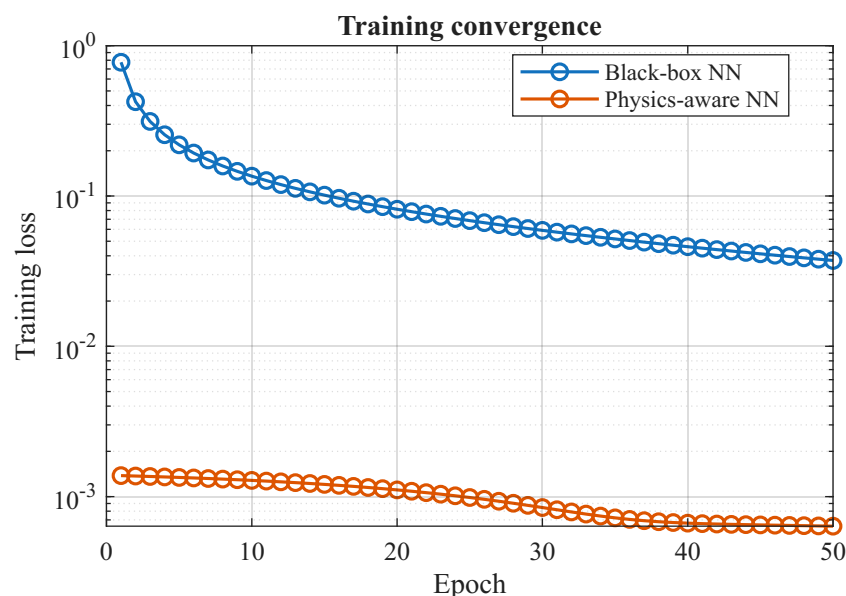
Figure 5. Training convergence for the black-box and physics-aware networks used in the constructive sparse SAR experiment. This diagnostic reports optimization behavior during learning and is not used as evidence of reconstruction superiority over the long-run classical baselines.
