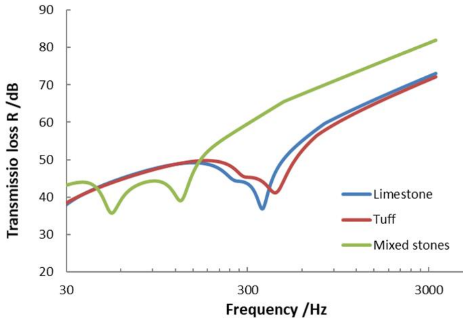
Figure 2: Empirical evaluations of the transmission loss of the 3 stone masonry partitions, with the proposed average values of the whole masonry wall high internal damping ( \eta_{int}^* \sim 10^{-1} ).
